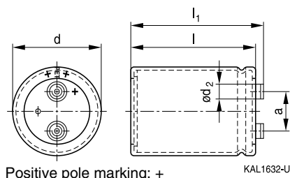
Ring clip/clamp mounting
