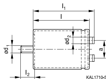
Threaded stud mounting
